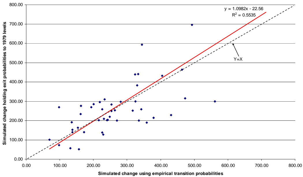
Scatter plot of simulated changes in state-level incarceration rates (1979 to 1998) holding exit probabilities constant against simulated changes using empirical transition probabilities
