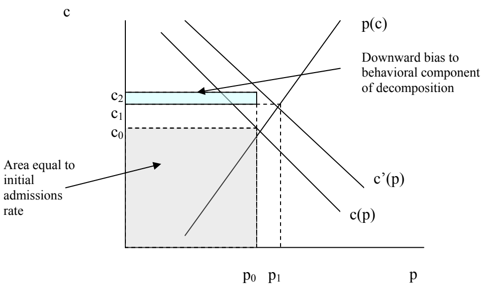
Figure 20: Demonstrating the Bias to the Behavioral Component of the Decomposition of Admissions Rates Due to Crimes Averted
